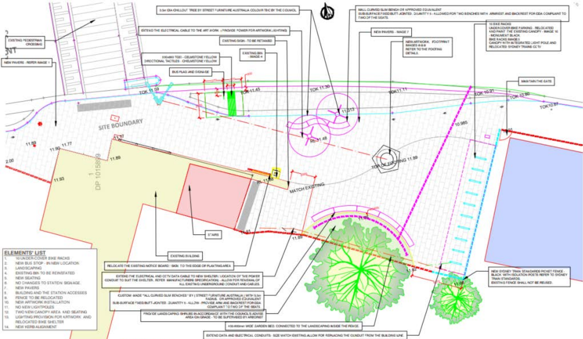
LAYOUT PLAN
